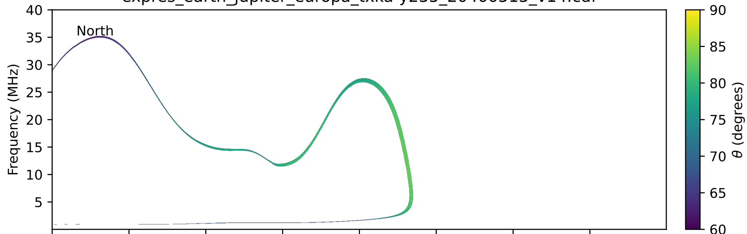
expres_earth_jupiter_europa_txka-y235_20400513_v14.cdf
