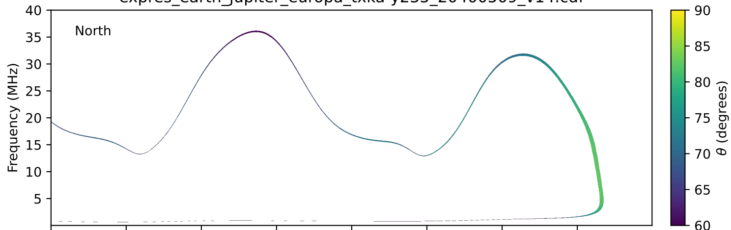
expres_earth_jupiter_europa_txka-y235_20400509_v14.cdf
