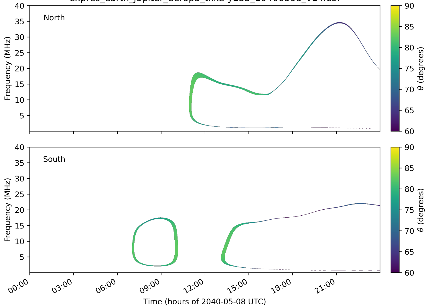
expres_earth_jupiter_europa_txka-y235_20400508_v14.cdf
