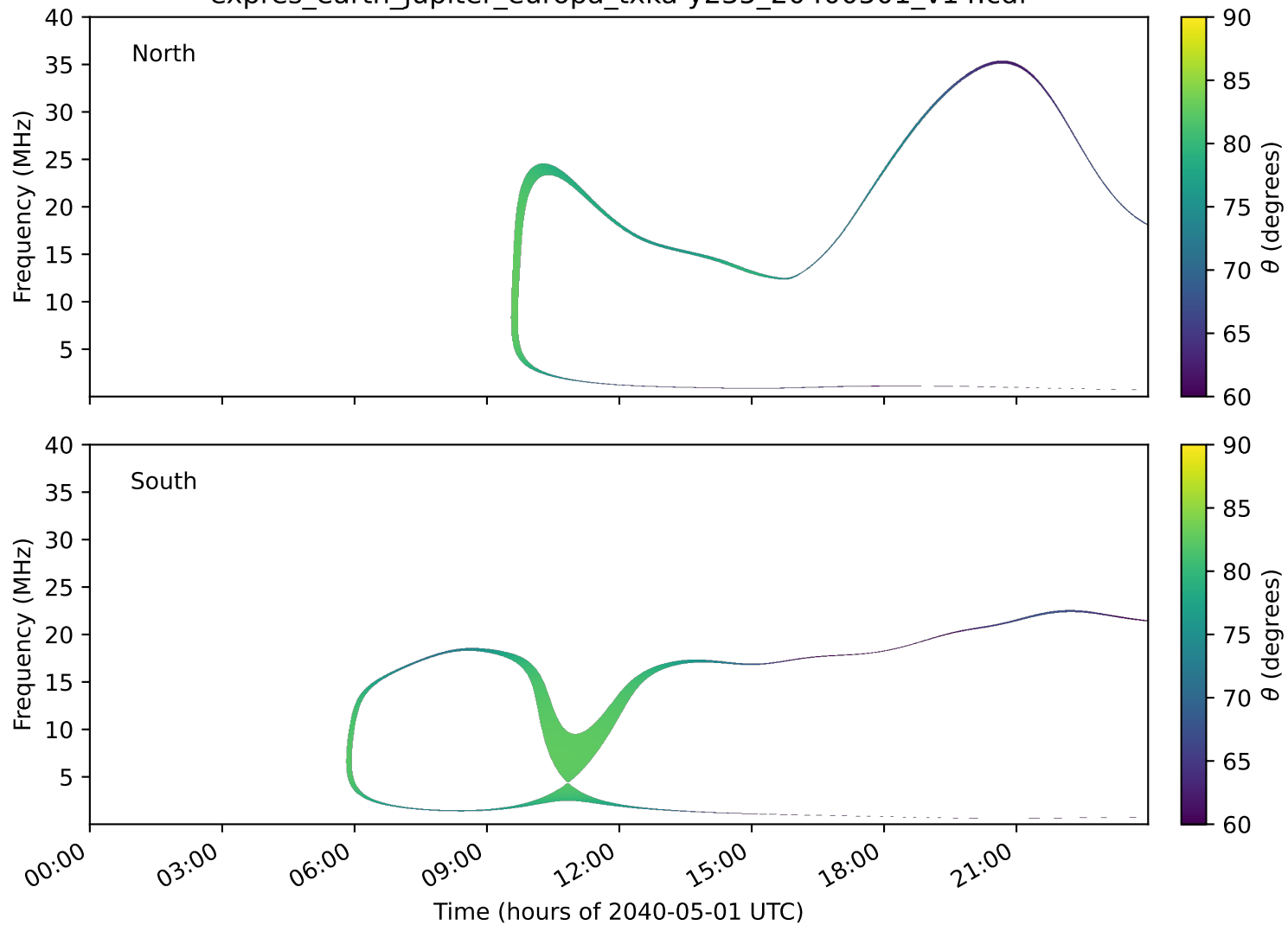
expres_earth_jupiter_europa_txka-y235_20400501_v14.cdf
