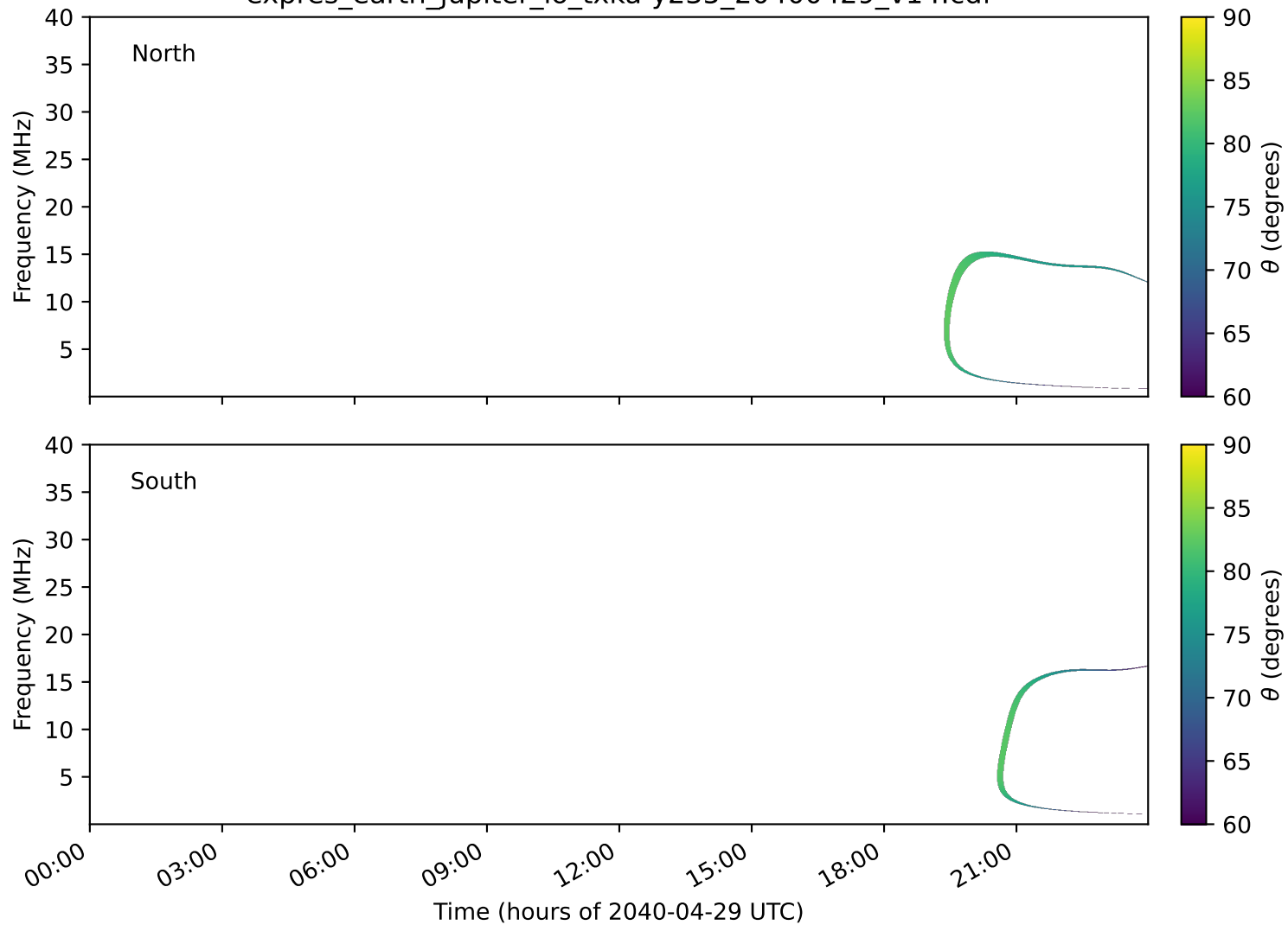
expres_earth_jupiter_io_txka-y235_20400429_v14.cdf
