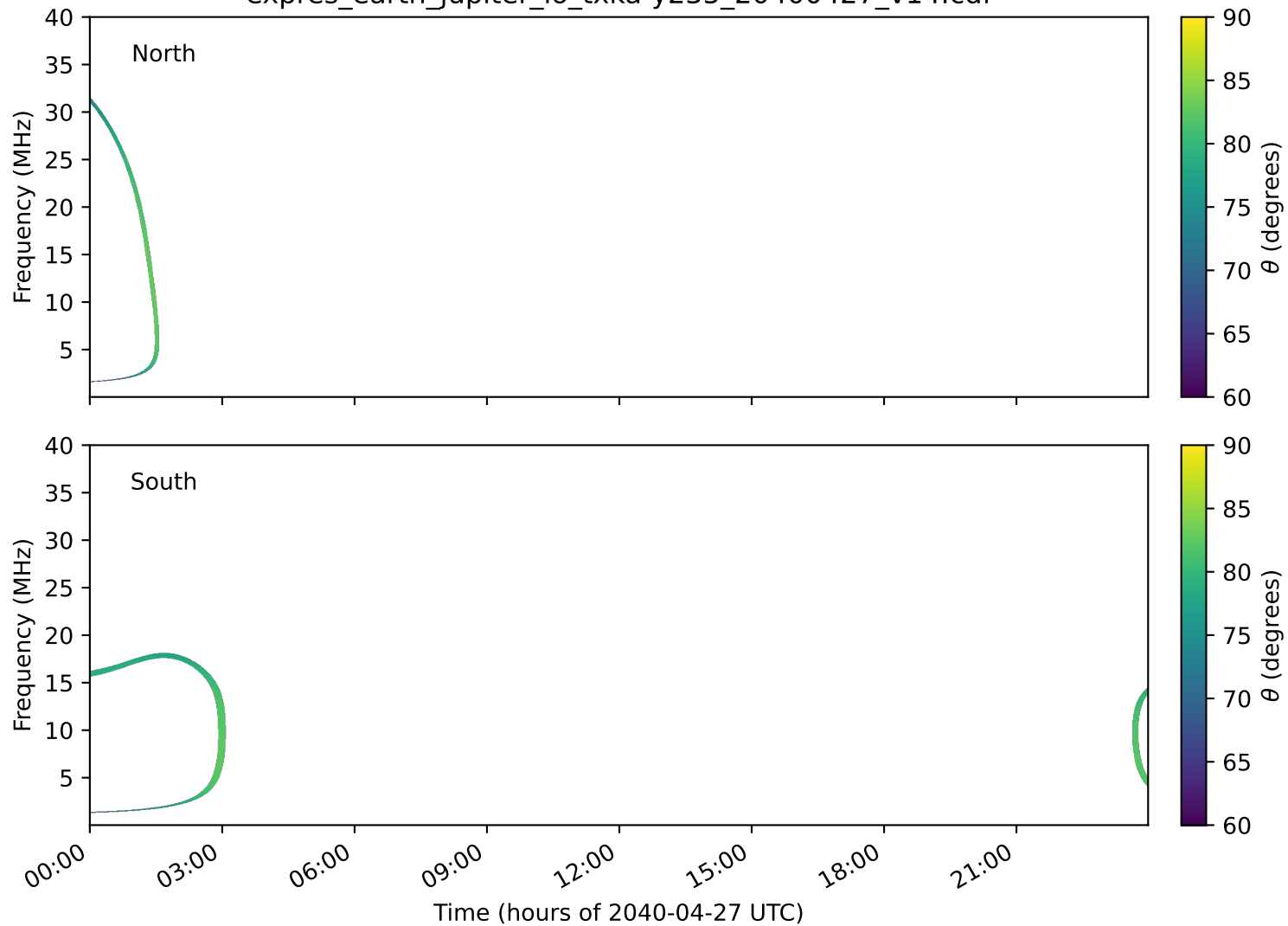
expres_earth_jupiter_io_txka-y235_20400427_v14.cdf
