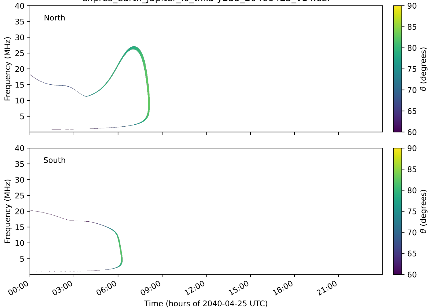
expres_earth_jupiter_io_txka-y235_20400425_v14.cdf
