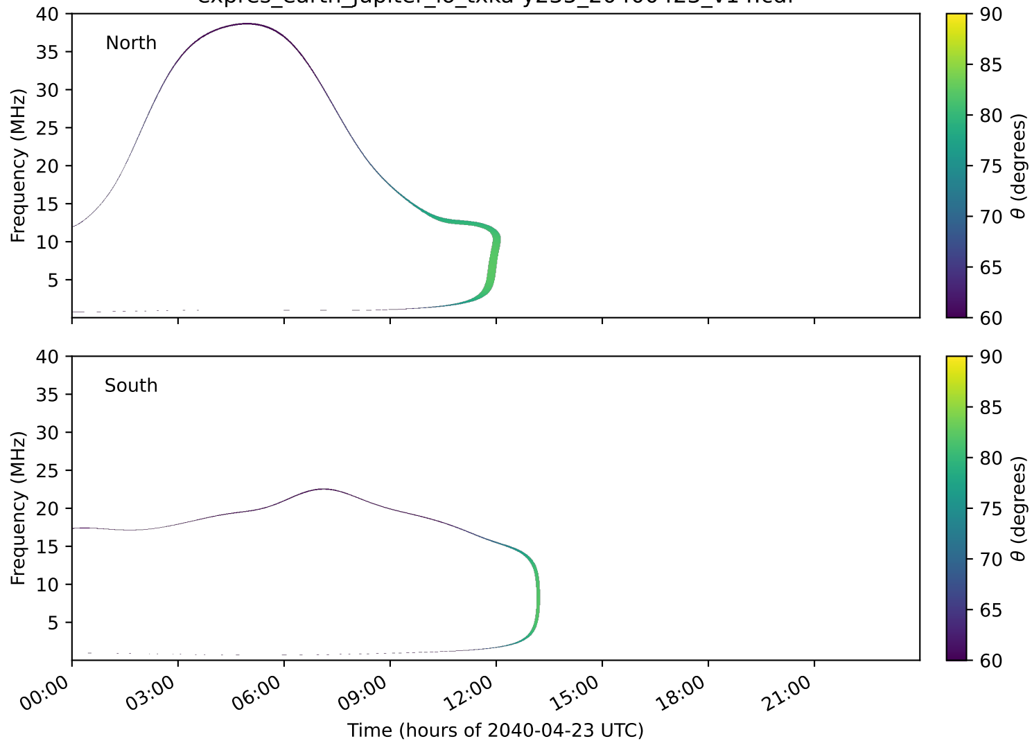
expres_earth_jupiter_io_txka-y235_20400423_v14.cdf
