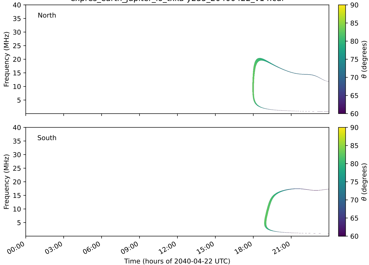
expres_earth_jupiter_io_txka-y235_20400422_v14.cdf
