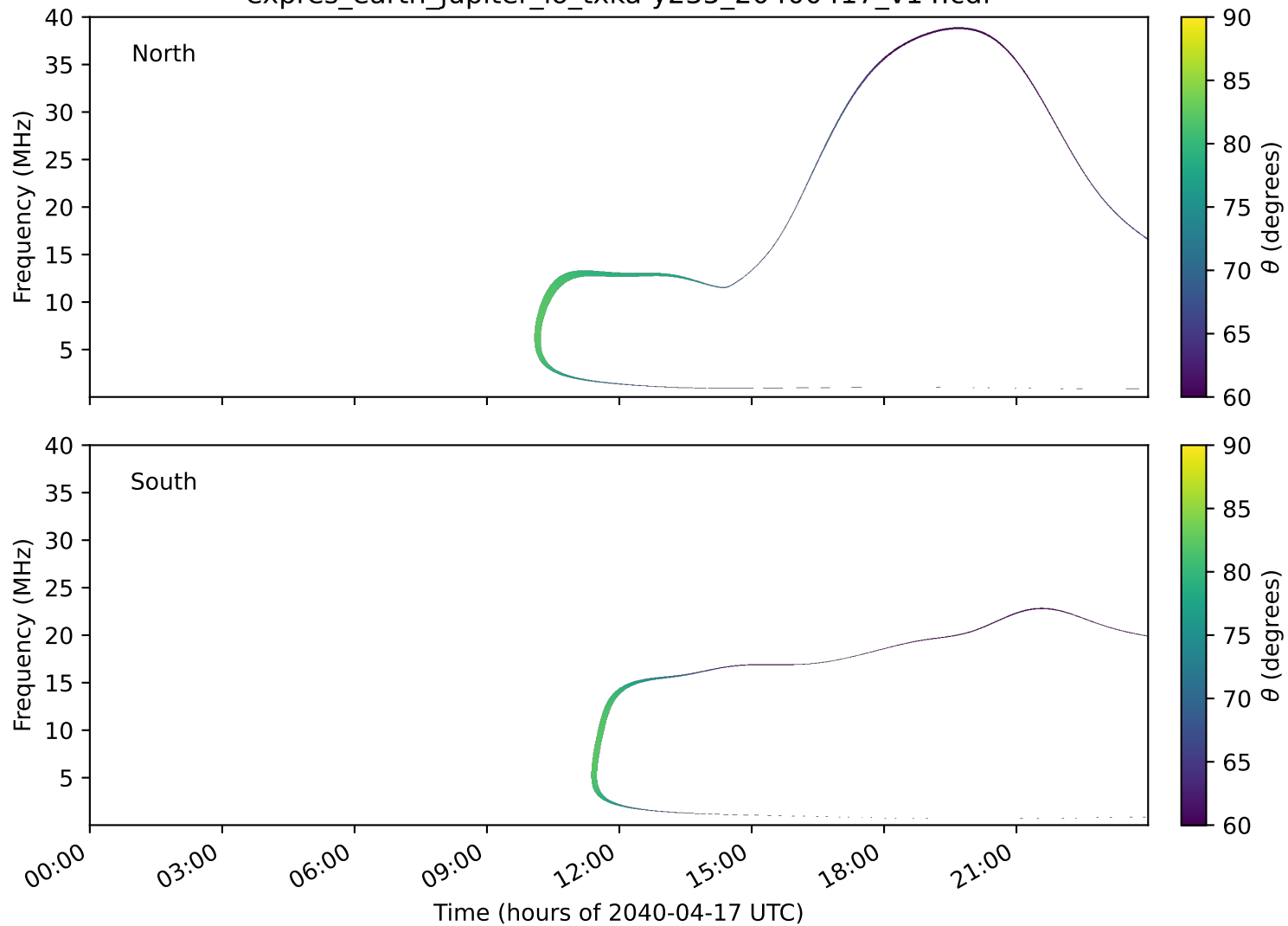
expres_earth_jupiter_io_txka-y235_20400417_v14.cdf
