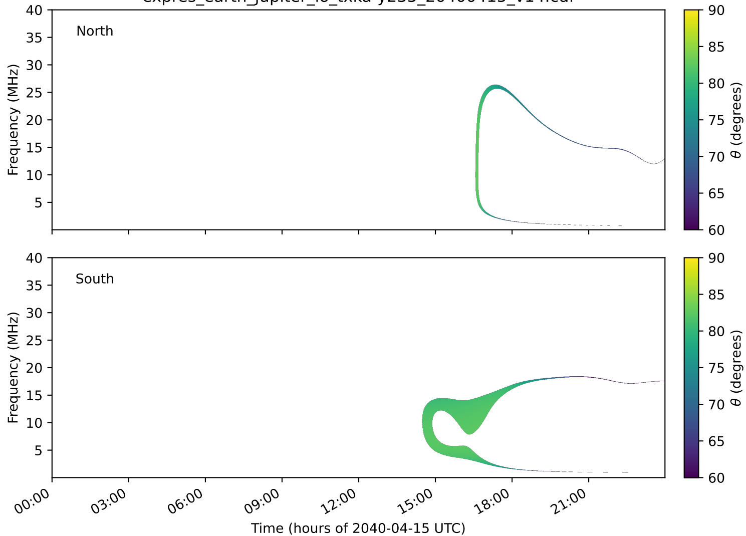
expres_earth_jupiter_io_txka-y235_20400415_v14.cdf
