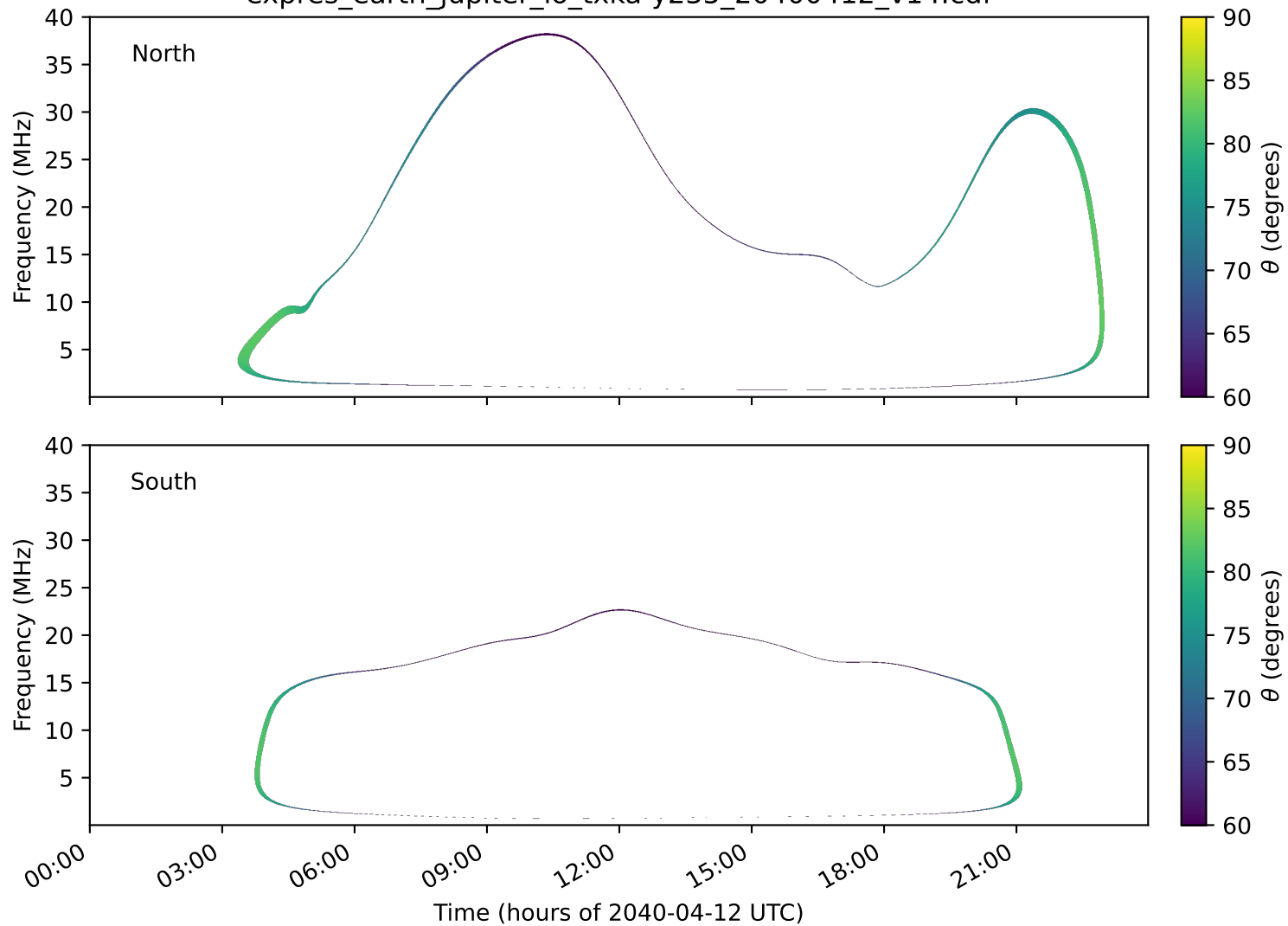
expres_earth_jupiter_io_txka-y235_20400412_v14.cdf
