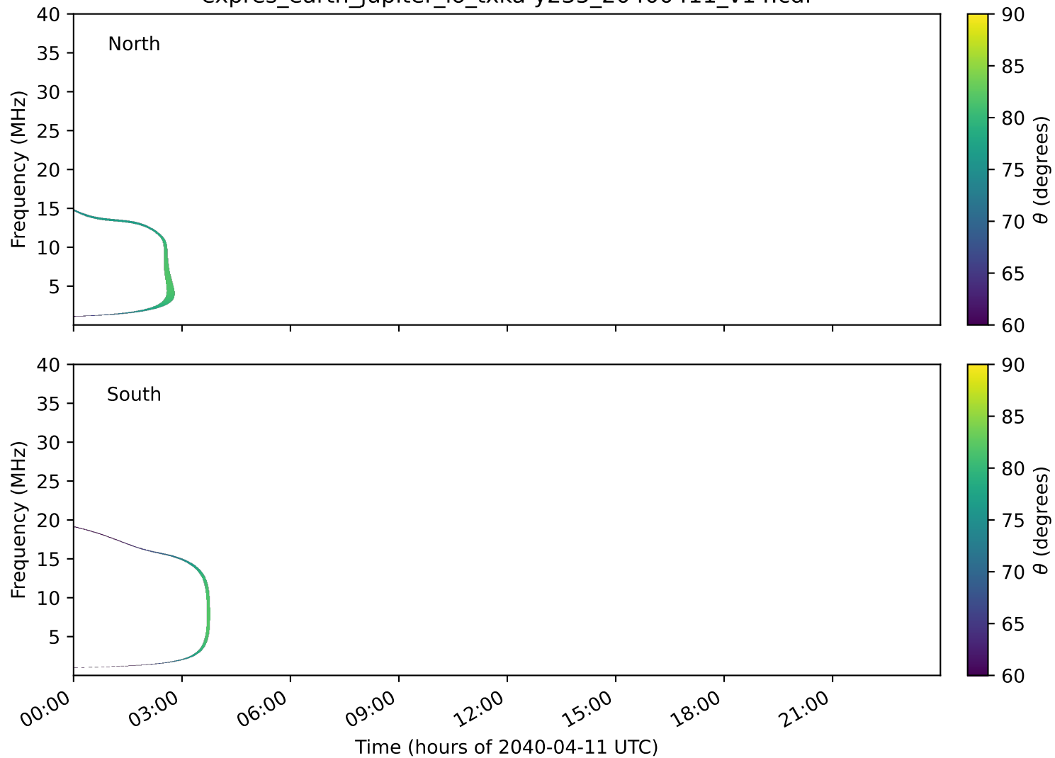
expres_earth_jupiter_io_txka-y235_20400411_v14.cdf
