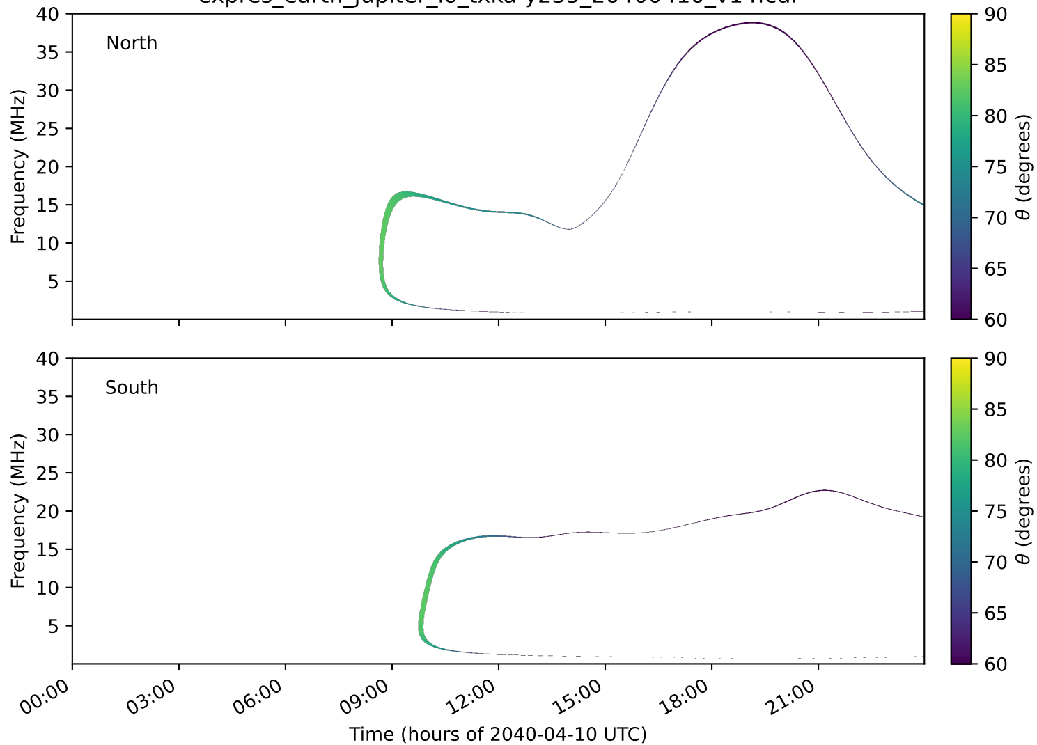
expres_earth_jupiter_io_txka-y235_20400410_v14.cdf
