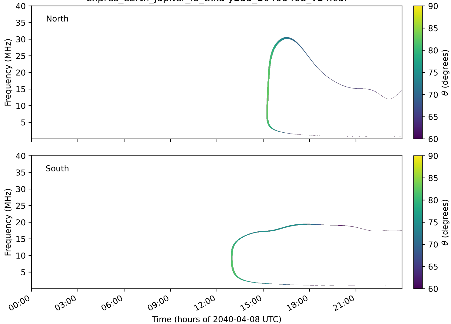
expres_earth_jupiter_io_txka-y235_20400408_v14.cdf
