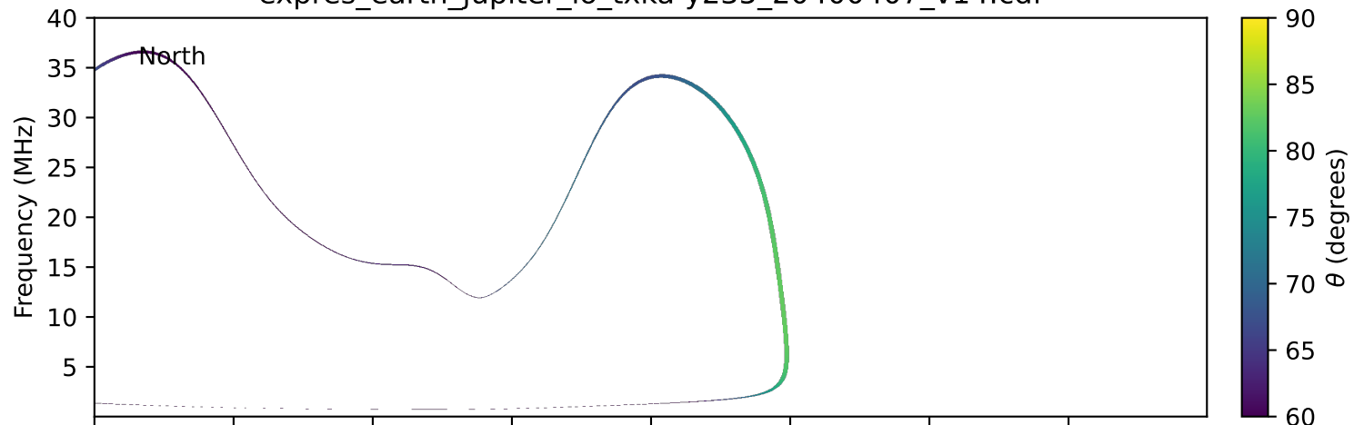
expres_earth_jupiter_io_txka-y235_20400407_v14.cdf
