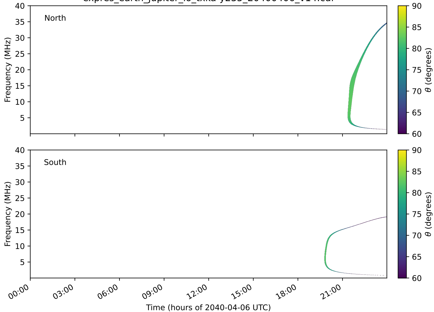
expres_earth_jupiter_io_txka-y235_20400406_v14.cdf
