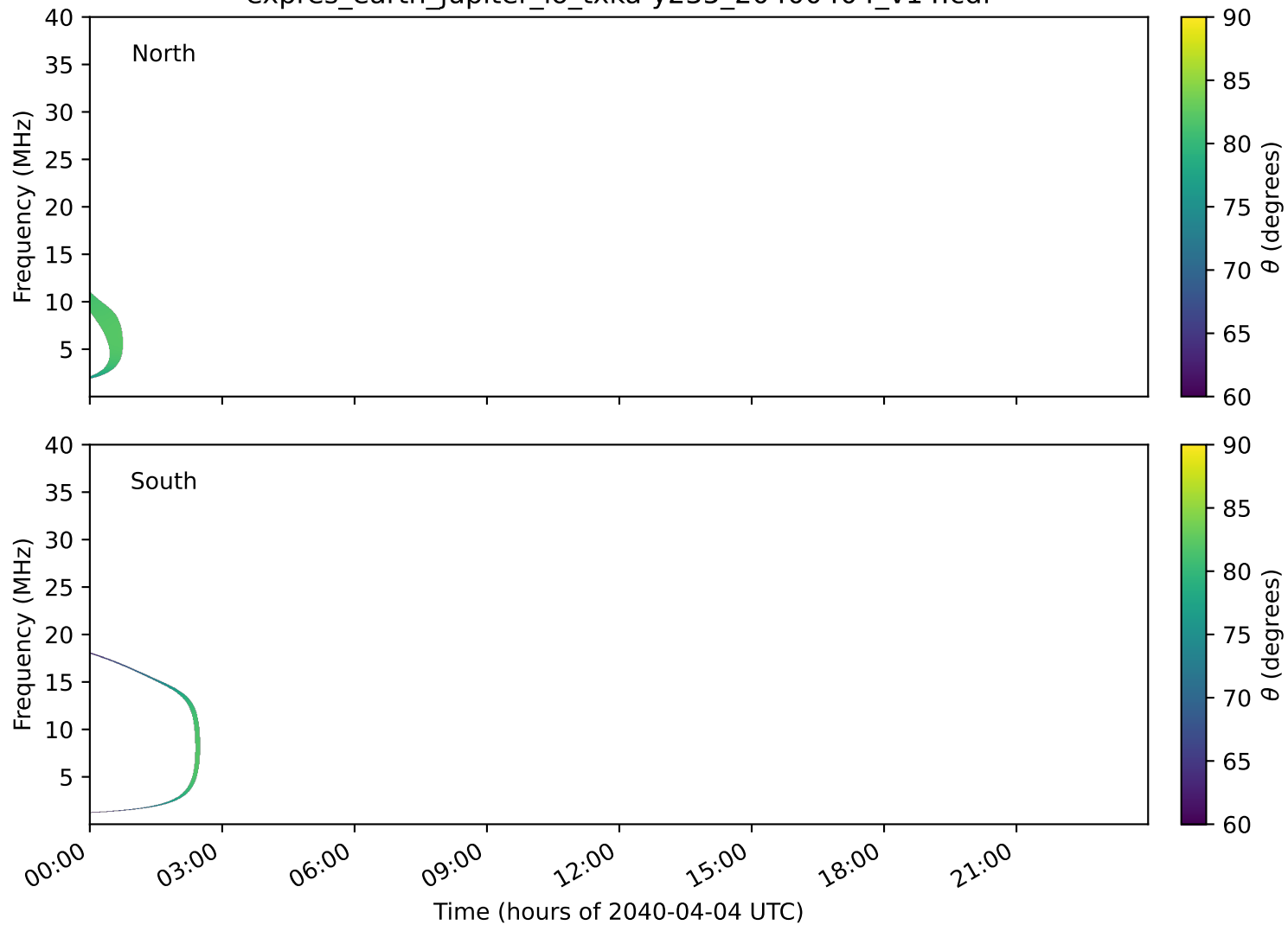
expres_earth_jupiter_io_txka-y235_20400404_v14.cdf
