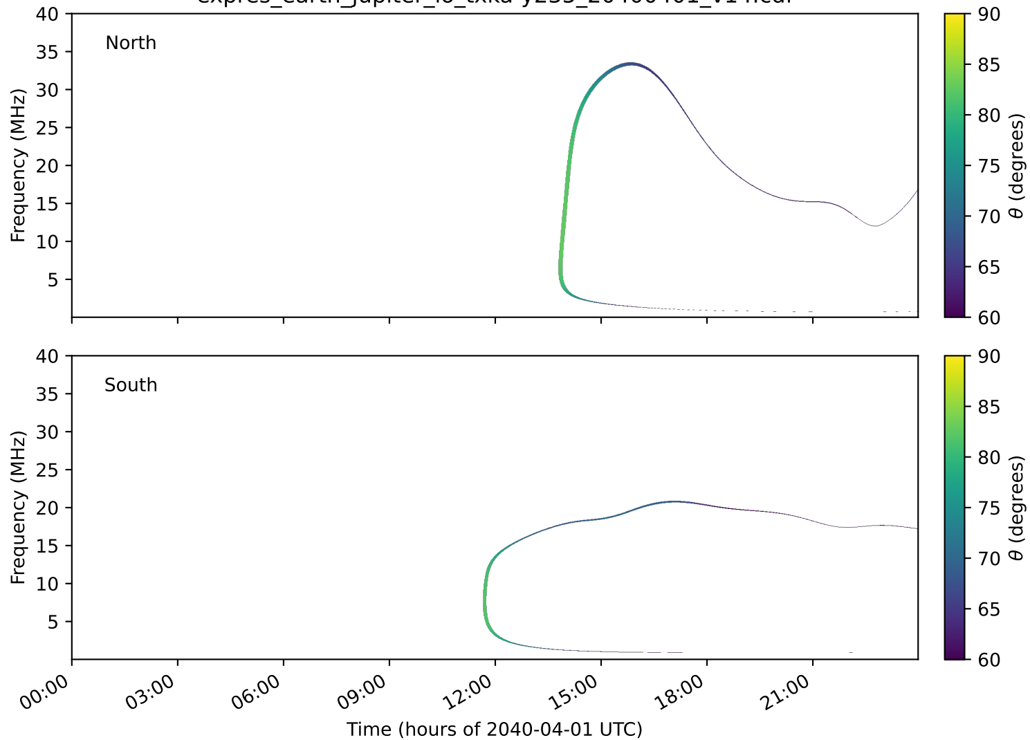
expres_earth_jupiter_io_txka-y235_20400401_v14.cdf
