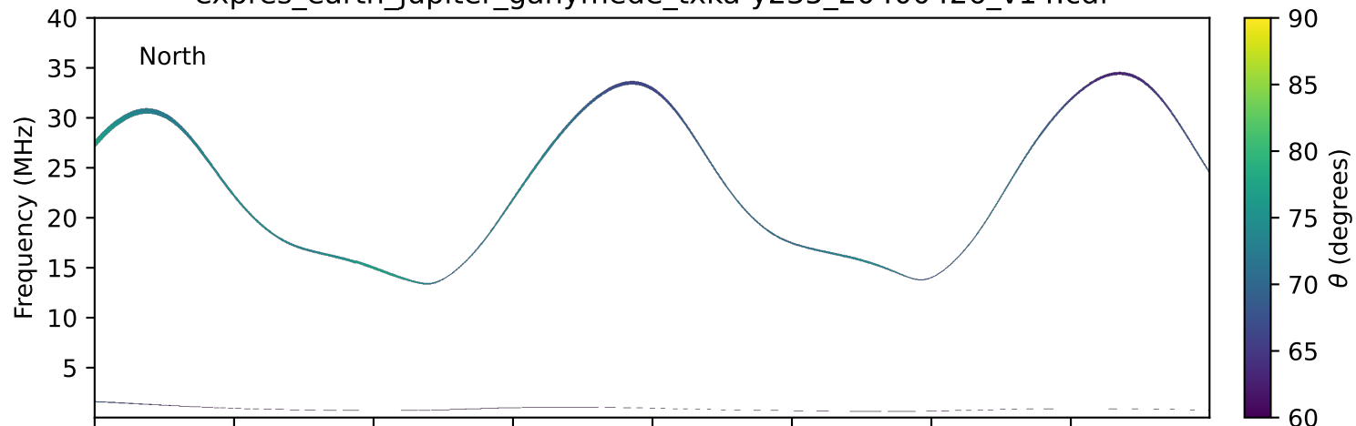
expres_earth_jupiter_ganymede_txka-y235_20400426_v14.cdf
