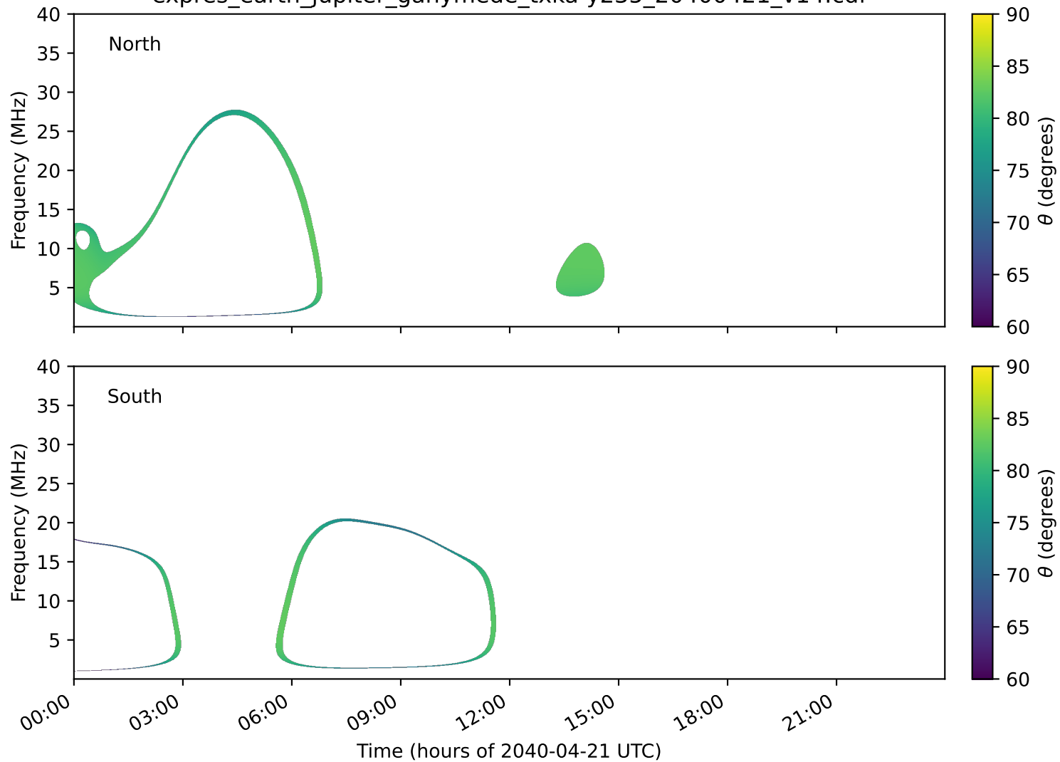
expres_earth_jupiter_ganymede_txka-y235_20400421_v14.cdf
