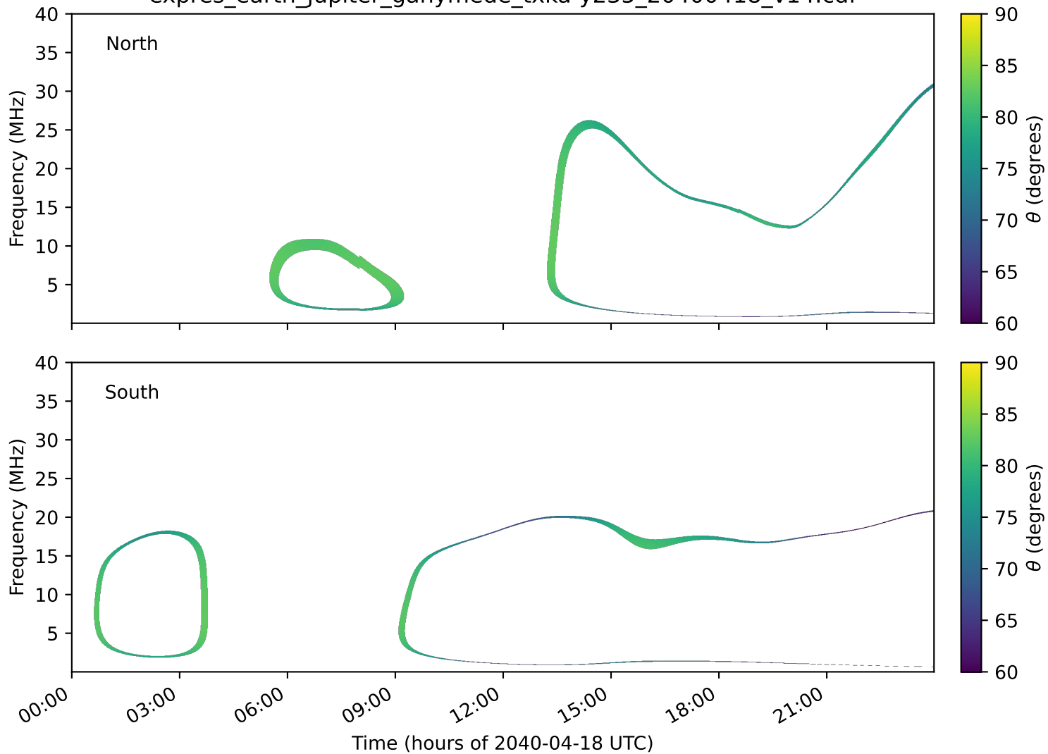
expres_earth_jupiter_ganymede_txka-y235_20400418_v14.cdf
