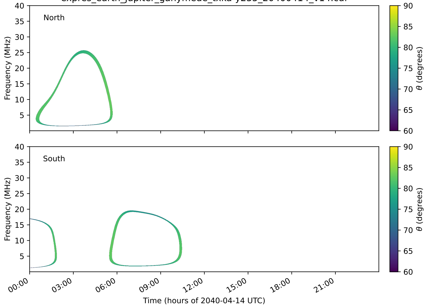
expres_earth_jupiter_ganymede_txka-y235_20400414_v14.cdf
