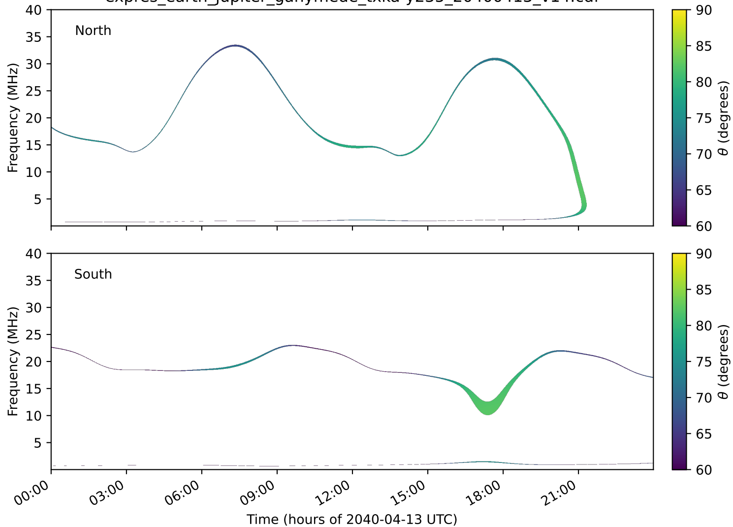
expres_earth_jupiter_ganymede_txka-y235_20400413_v14.cdf
