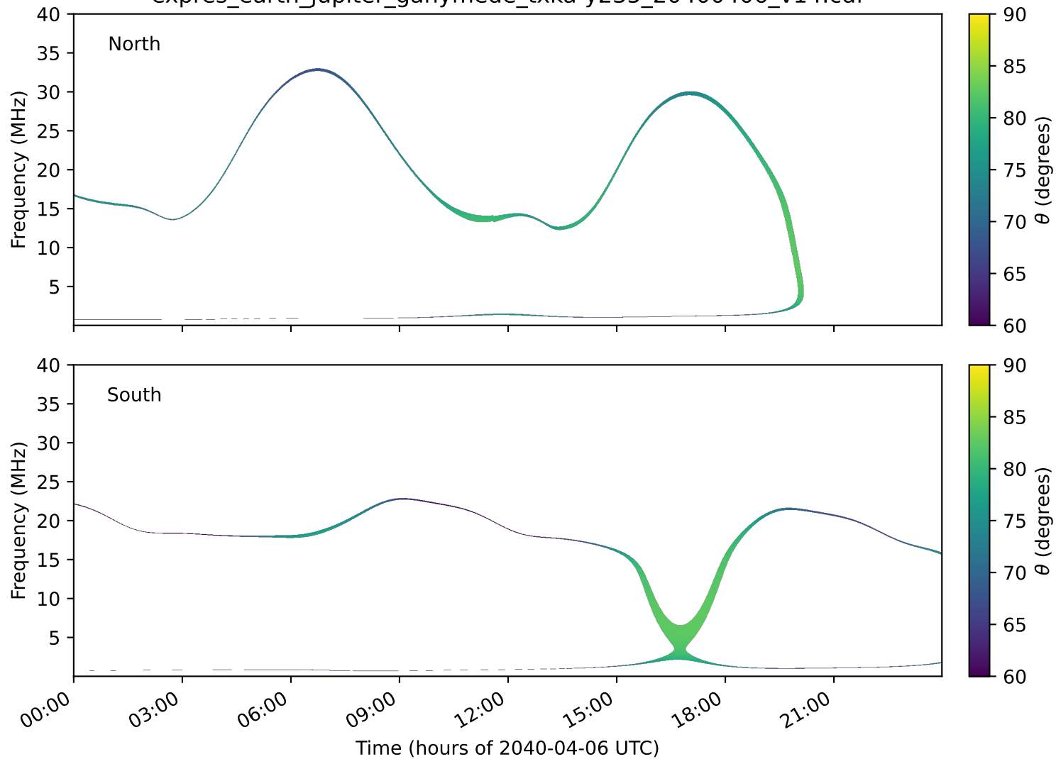
expres_earth_jupiter_ganymede_txka-y235_20400406_v14.cdf
