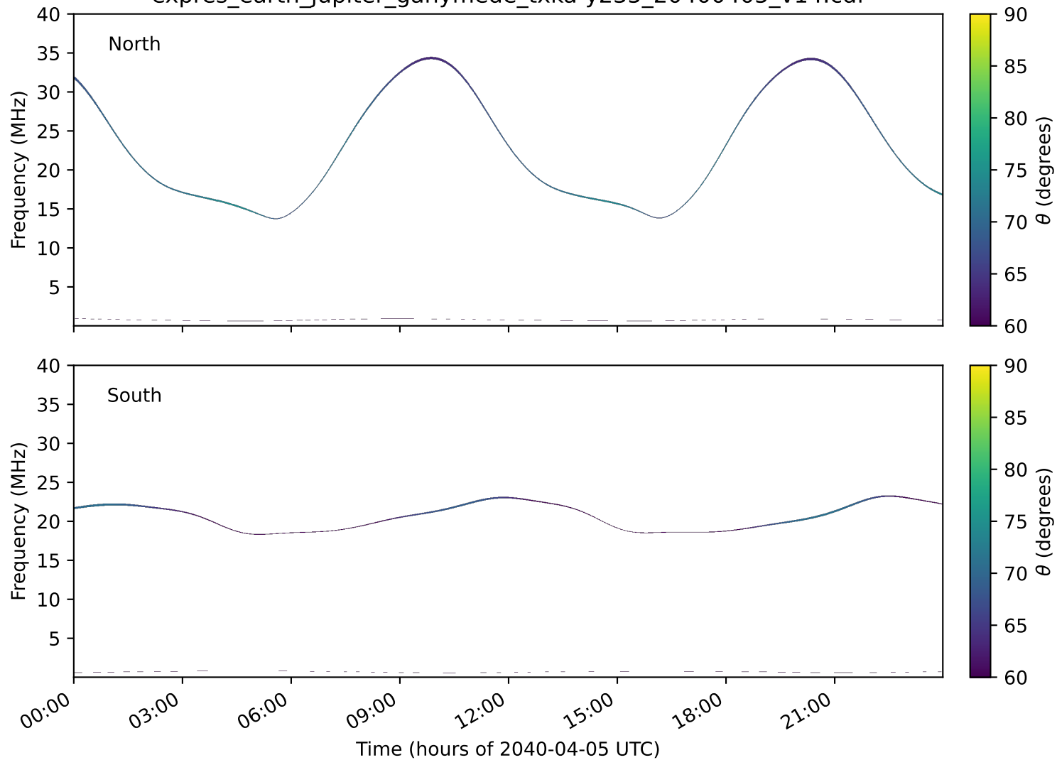
expres_earth_jupiter_ganymede_txka-y235_20400405_v14.cdf
