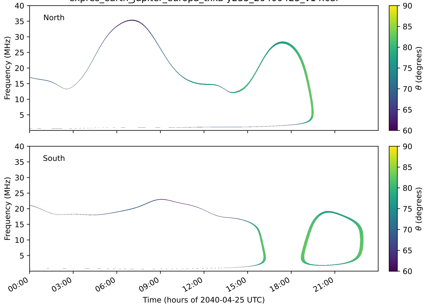
expres_earth_jupiter_europa_txka-y235_20400425_v14.cdf
