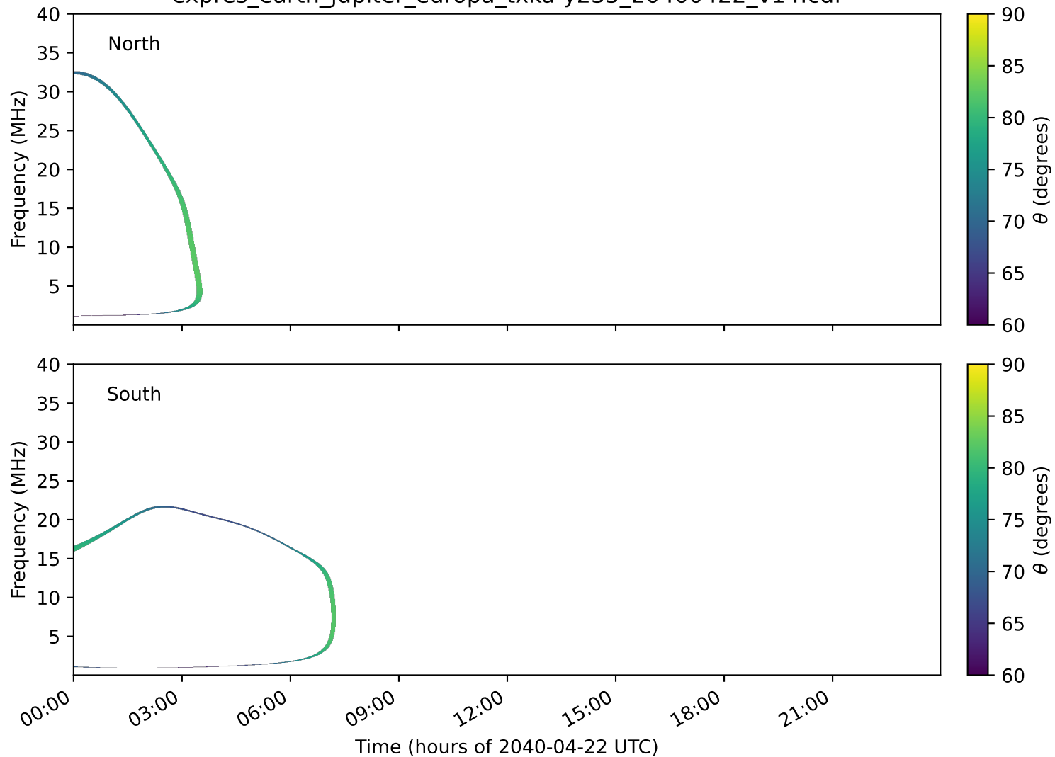
expres_earth_jupiter_europa_txka-y235_20400422_v14.cdf
