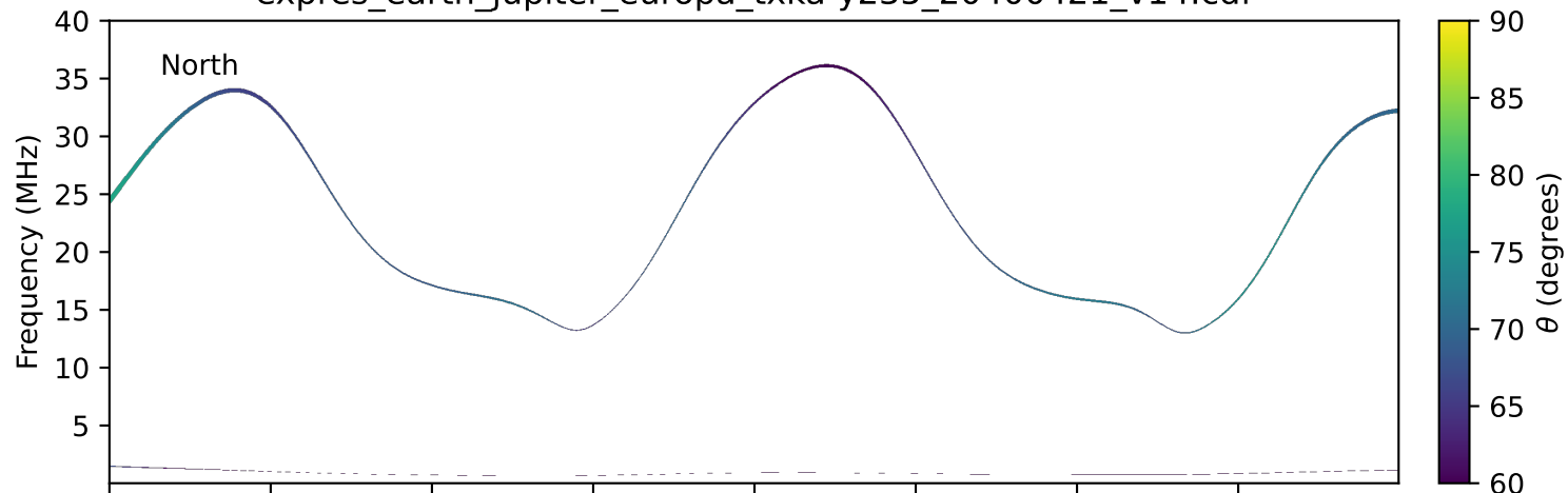
expres_earth_jupiter_europa_txka-y235_20400421_v14.cdf
