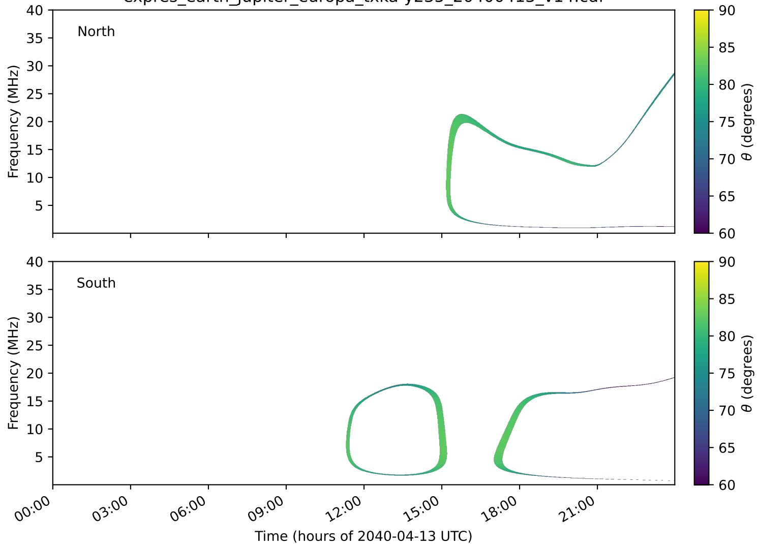
expres_earth_jupiter_europa_txka-y235_20400413_v14.cdf
