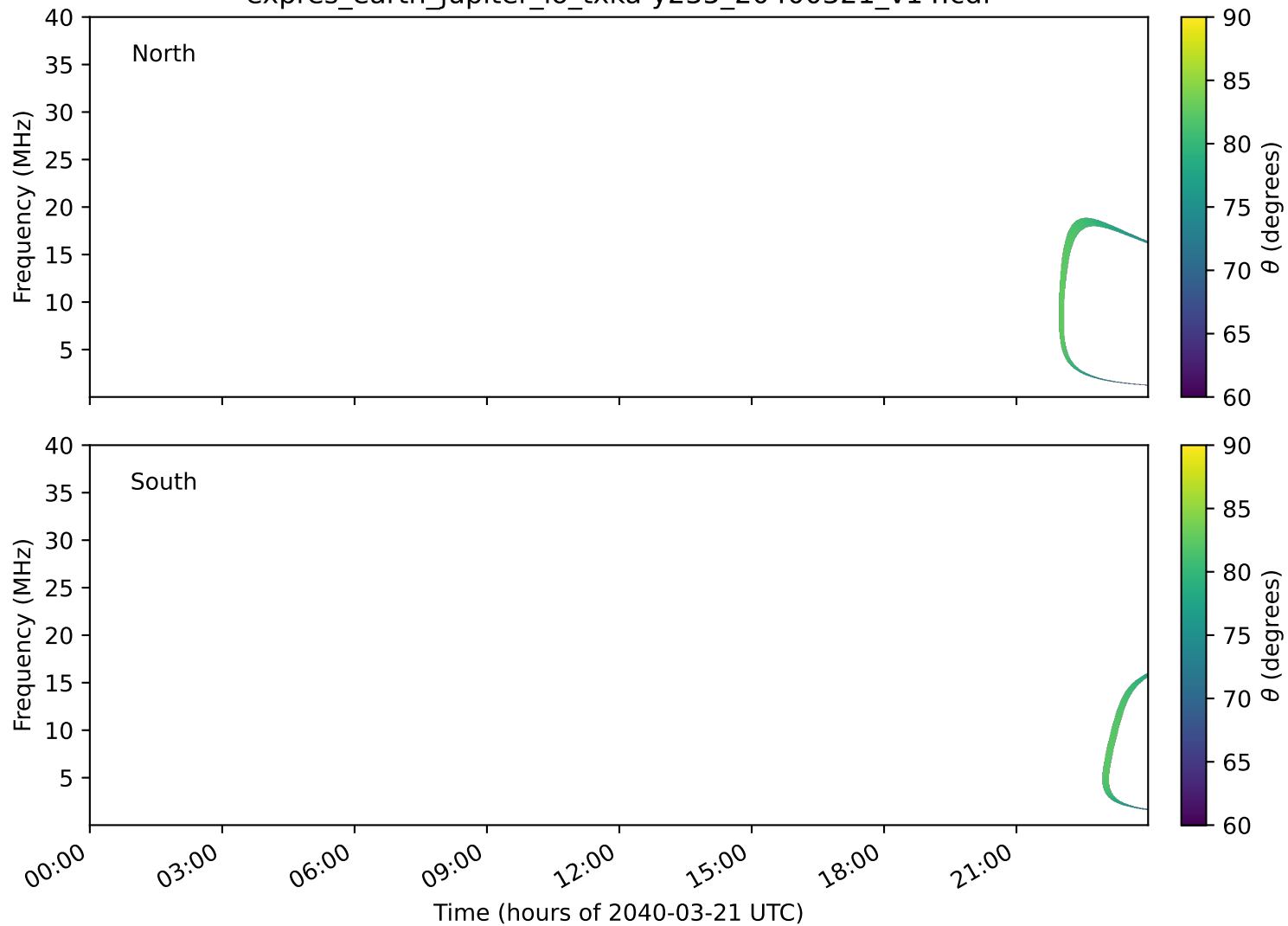
expres_earth_jupiter_io_txka-y235_20400321_v14.cdf
