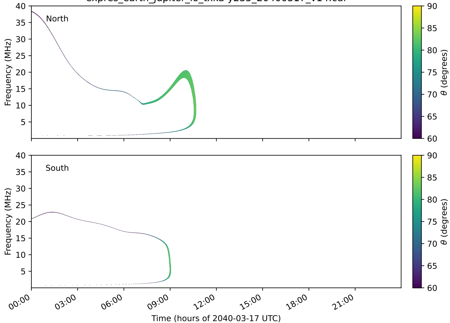
expres_earth_jupiter_io_txka-y235_20400317_v14.cdf
