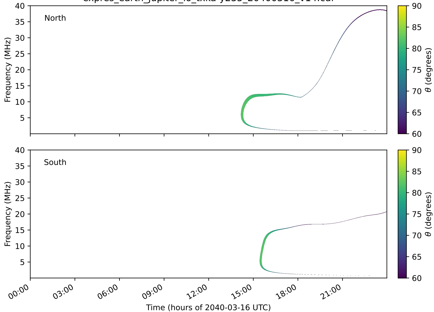
expres_earth_jupiter_io_txka-y235_20400316_v14.cdf
