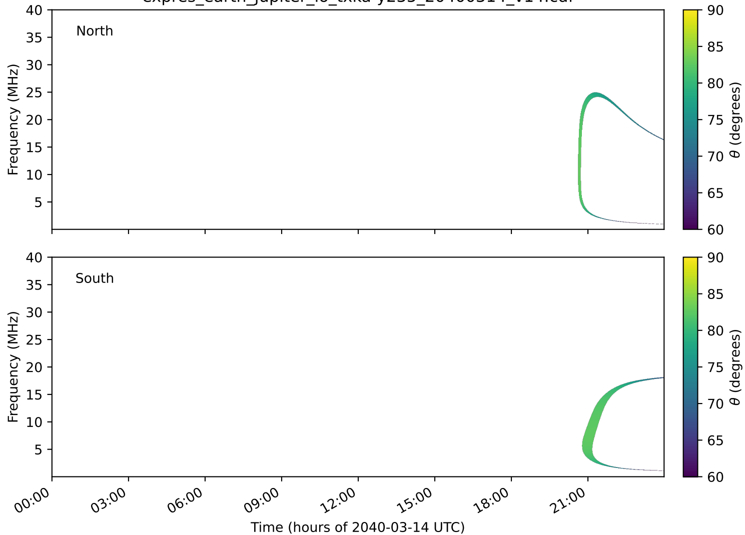
expres_earth_jupiter_io_txka-y235_20400314_v14.cdf
