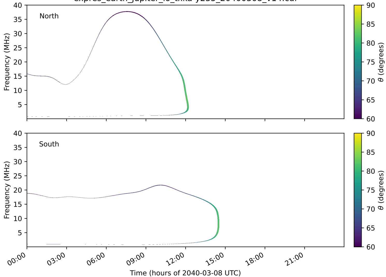
expres_earth_jupiter_io_txka-y235_20400308_v14.cdf
