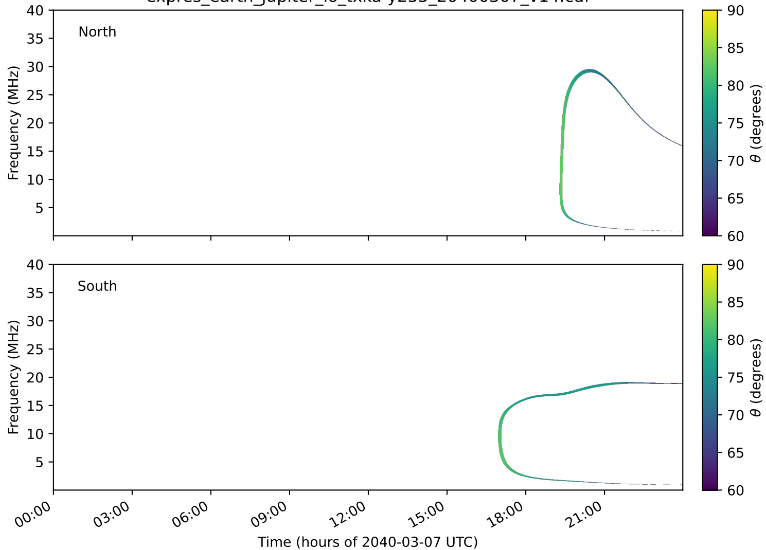
expres_earth_jupiter_io_txka-y235_20400307_v14.cdf
