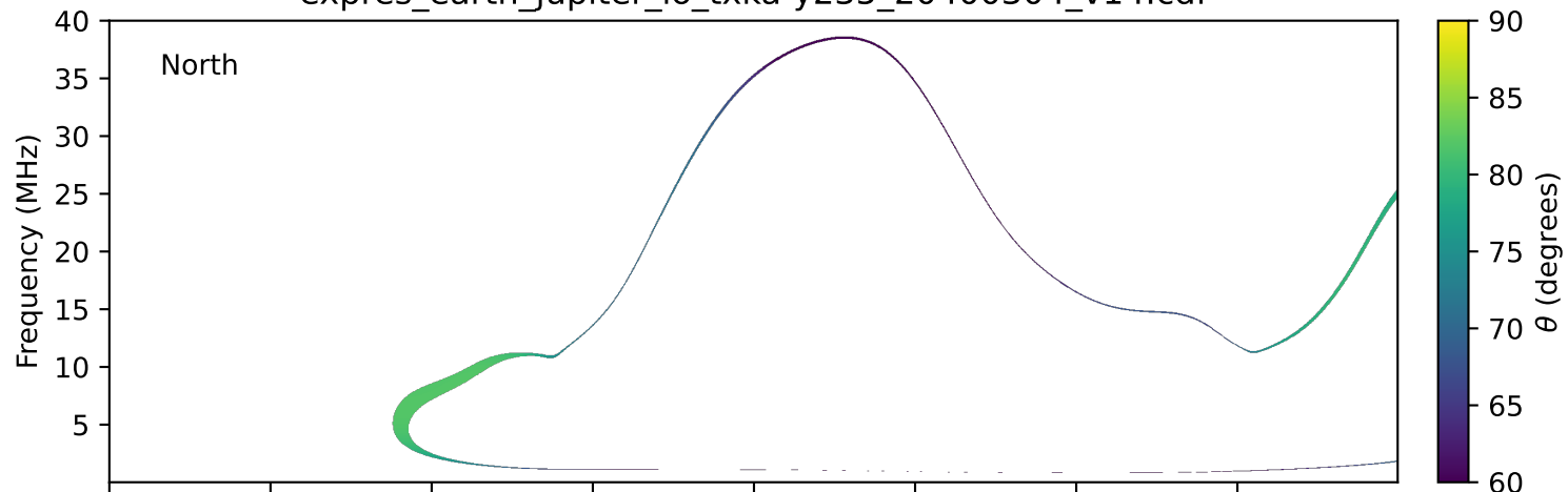
expres_earth_jupiter_io_txka-y235_20400304_v14.cdf
