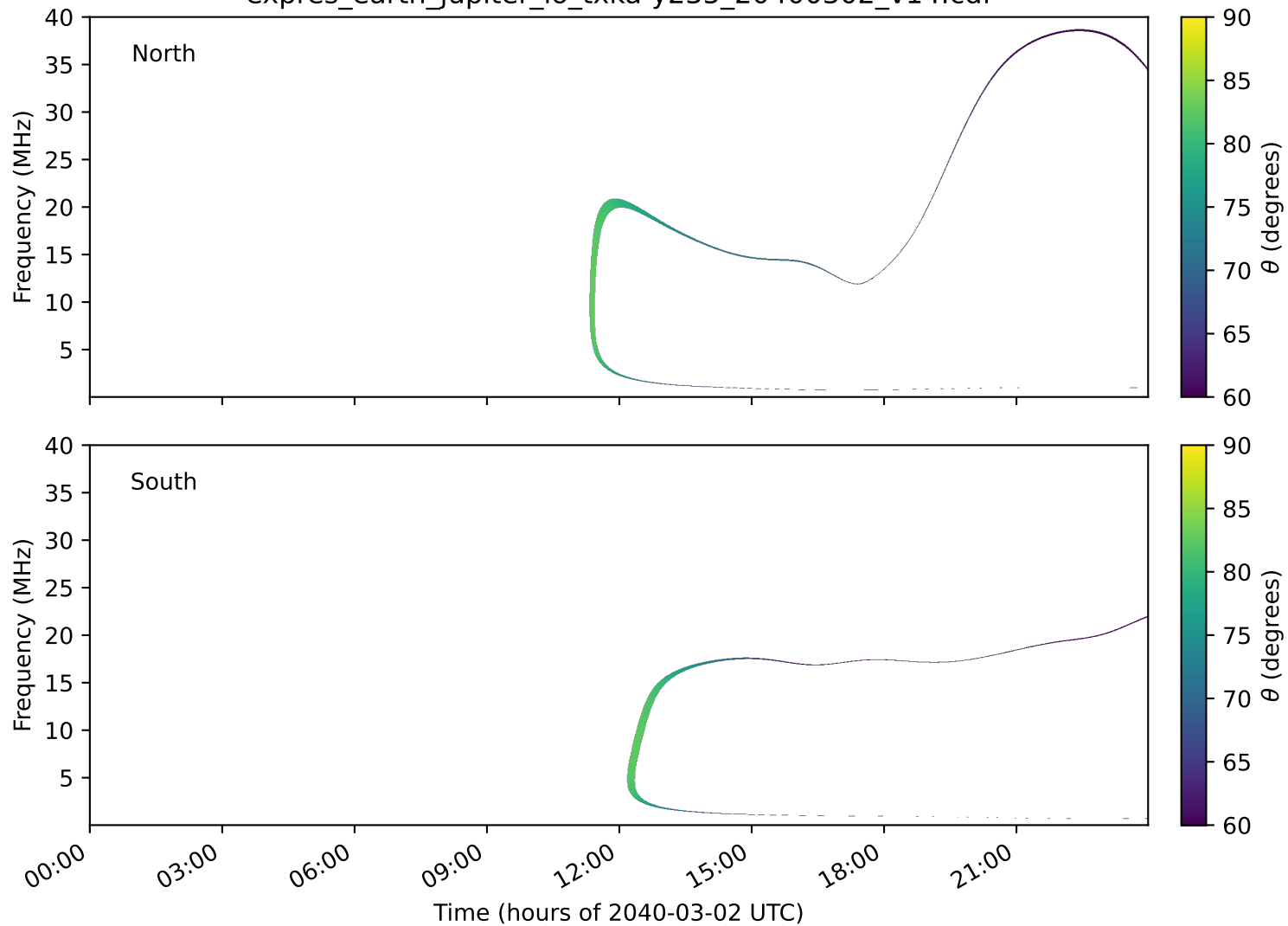
expres_earth_jupiter_io_txka-y235_20400302_v14.cdf
