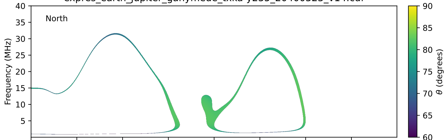
expres_earth_jupiter_ganymede_txka-y235_20400323_v14.cdf
