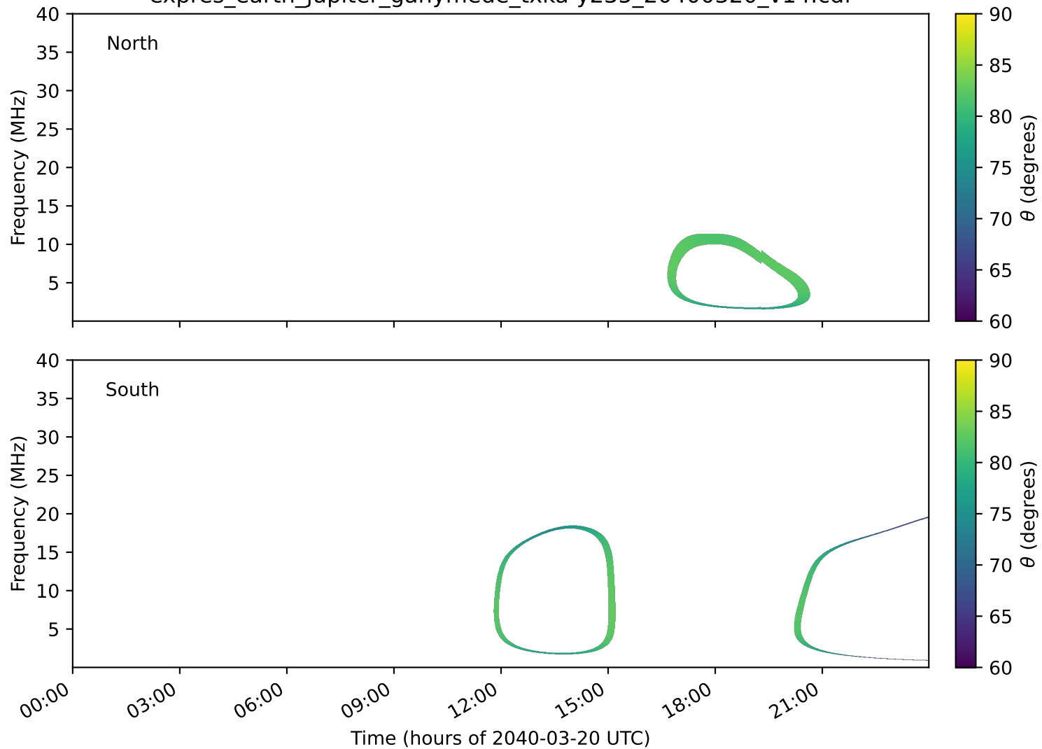
expres_earth_jupiter_ganymede_txka-y235_20400320_v14.cdf
