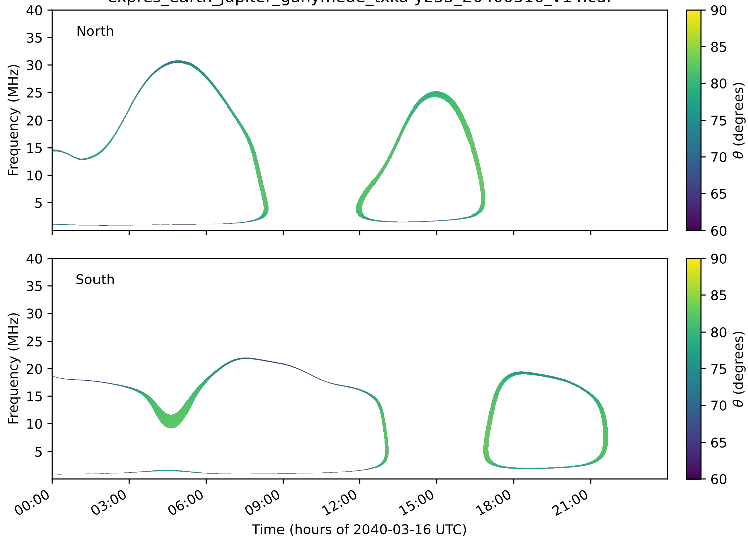
expres_earth_jupiter_ganymede_txka-y235_20400316_v14.cdf
