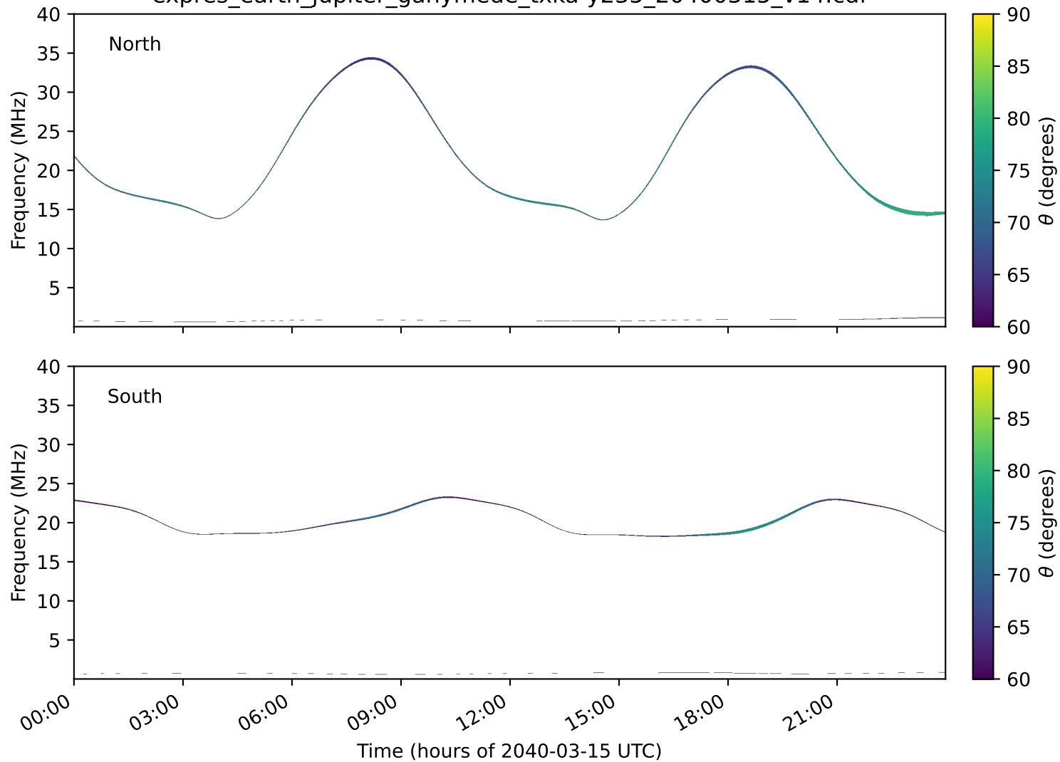
expres_earth_jupiter_ganymede_txka-y235_20400315_v14.cdf
