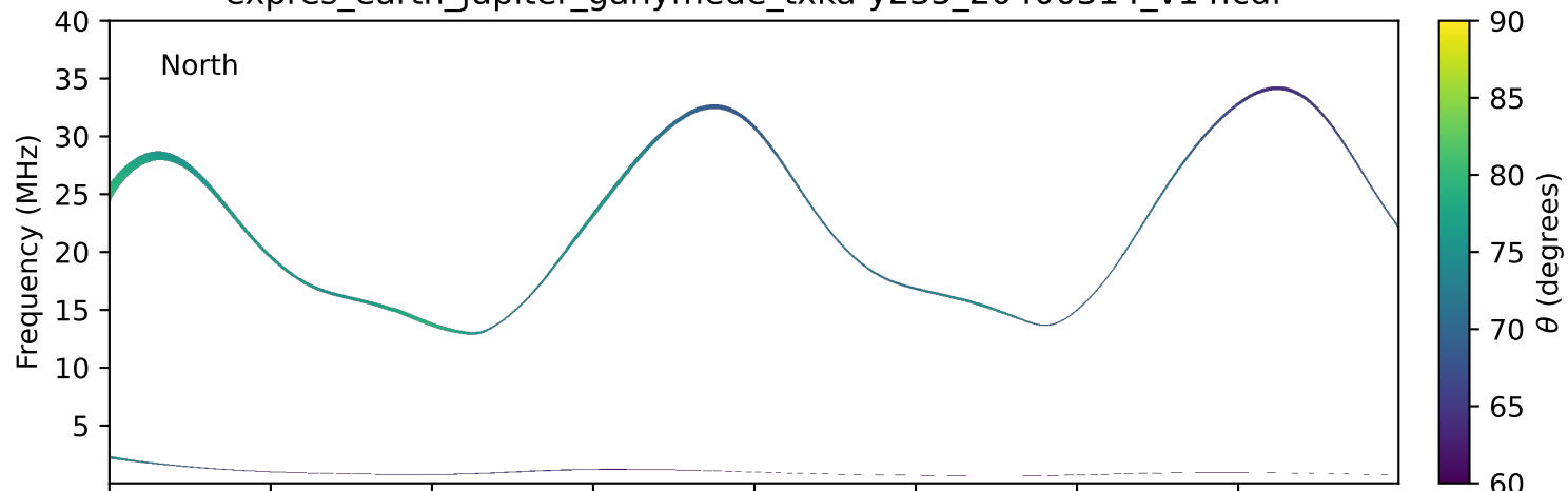
expres_earth_jupiter_ganymede_txka-y235_20400314_v14.cdf
