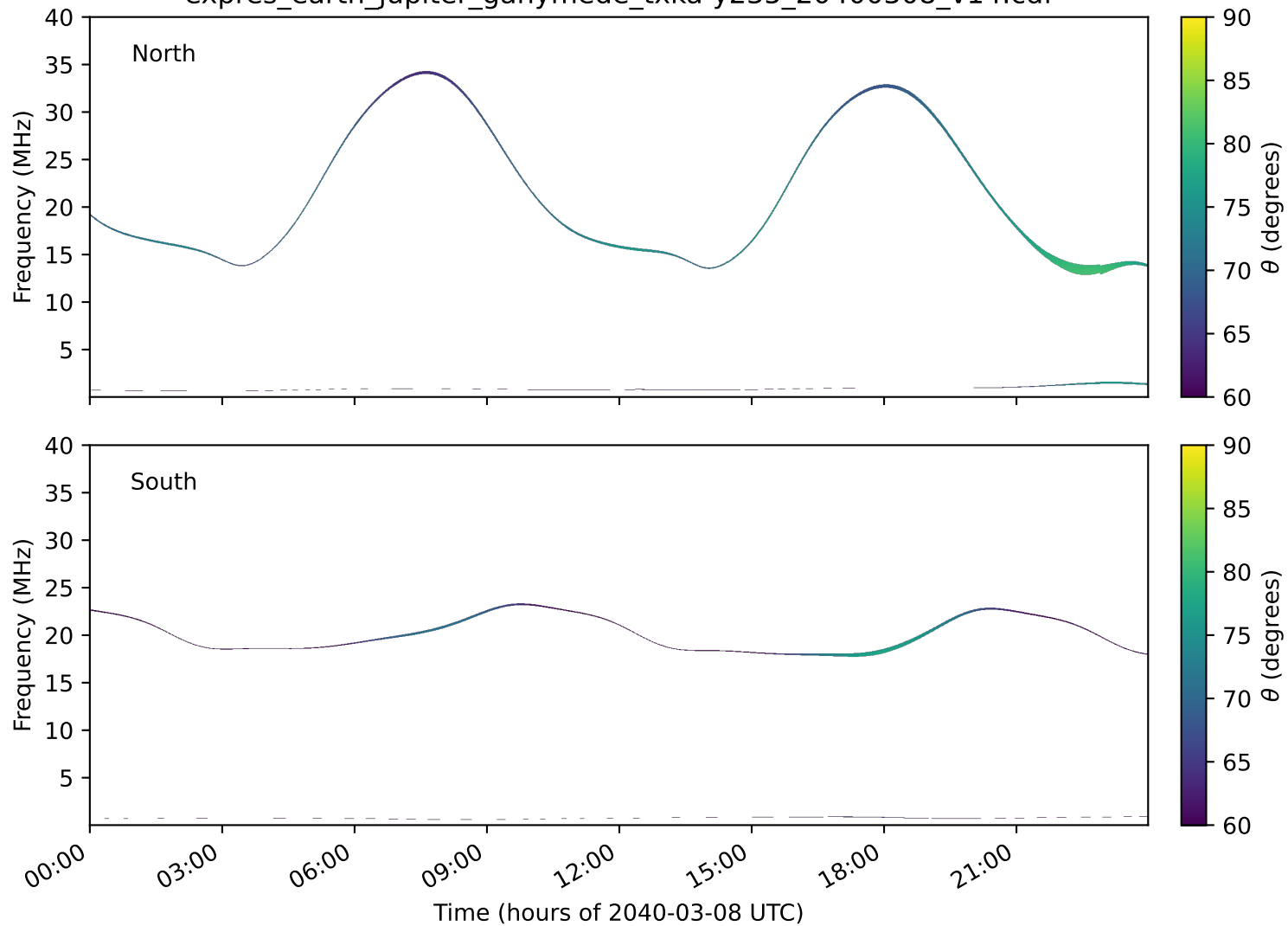
expres_earth_jupiter_ganymede_txka-y235_20400308_v14.cdf
