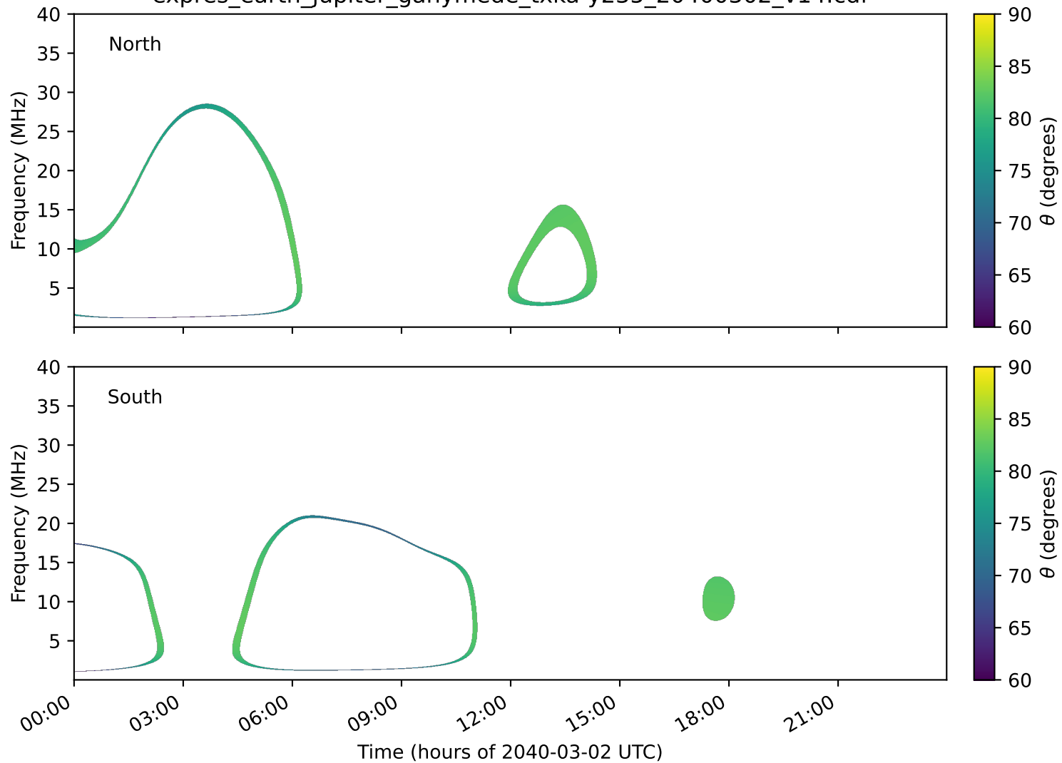
expres_earth_jupiter_ganymede_txka-y235_20400302_v14.cdf
