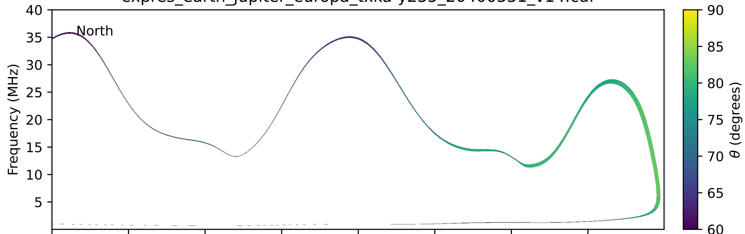
expres_earth_jupiter_europa_txka-y235_20400331_v14.cdf
