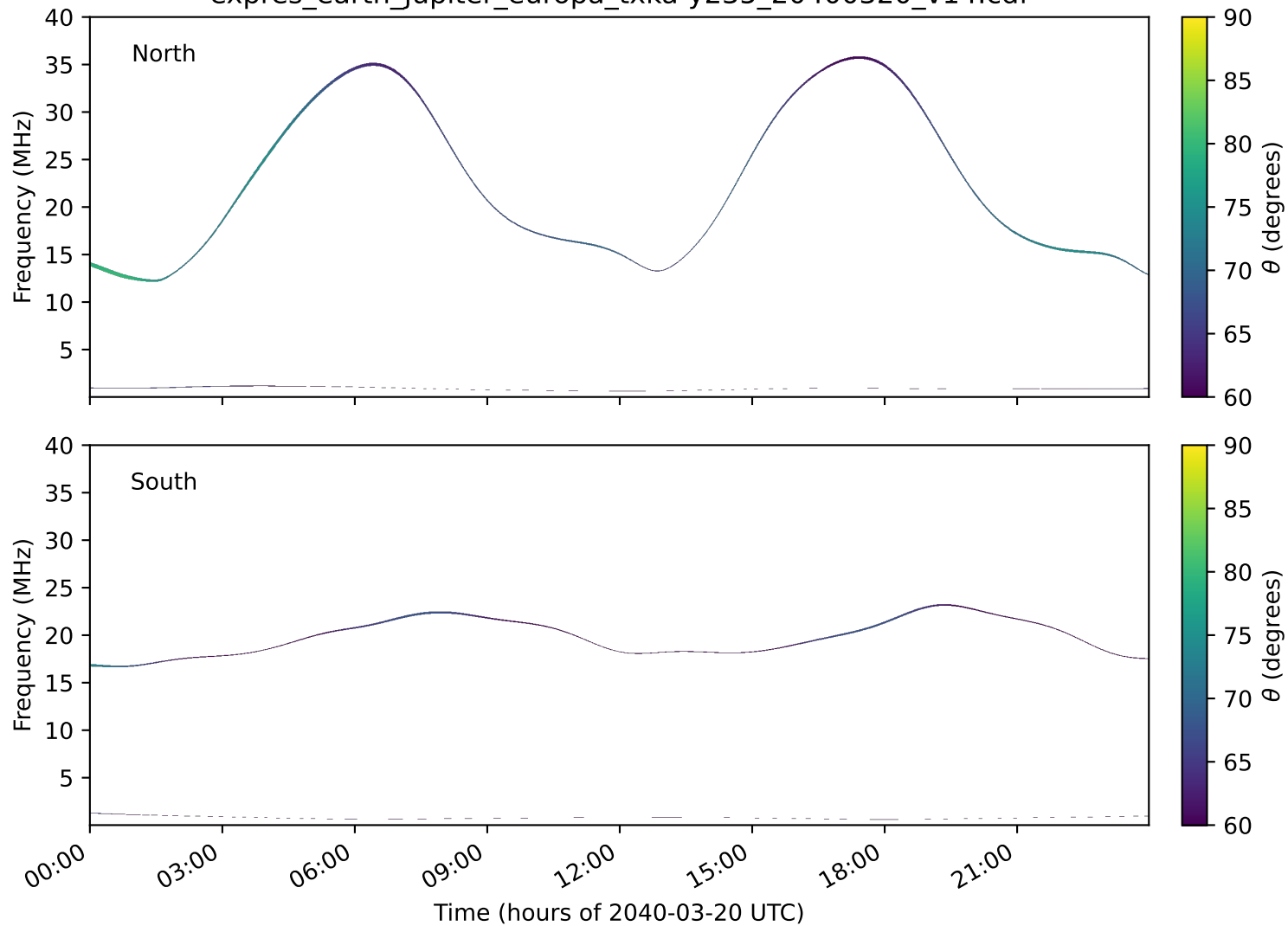
expres_earth_jupiter_europa_txka-y235_20400320_v14.cdf
