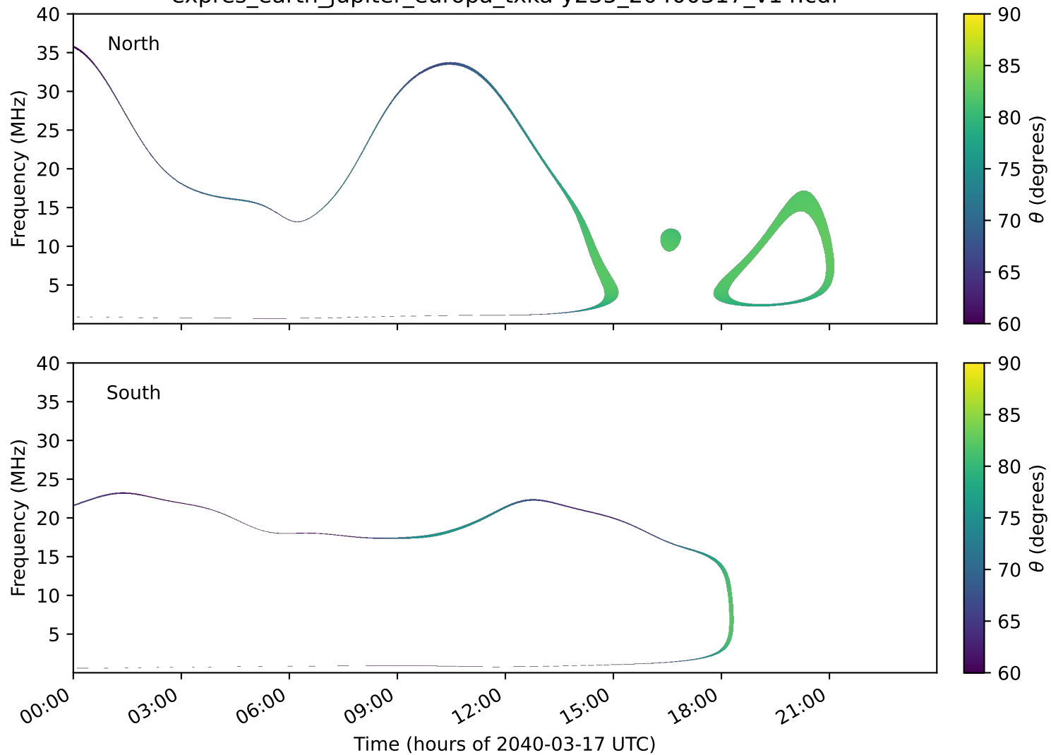
expres_earth_jupiter_europa_txka-y235_20400317_v14.cdf
