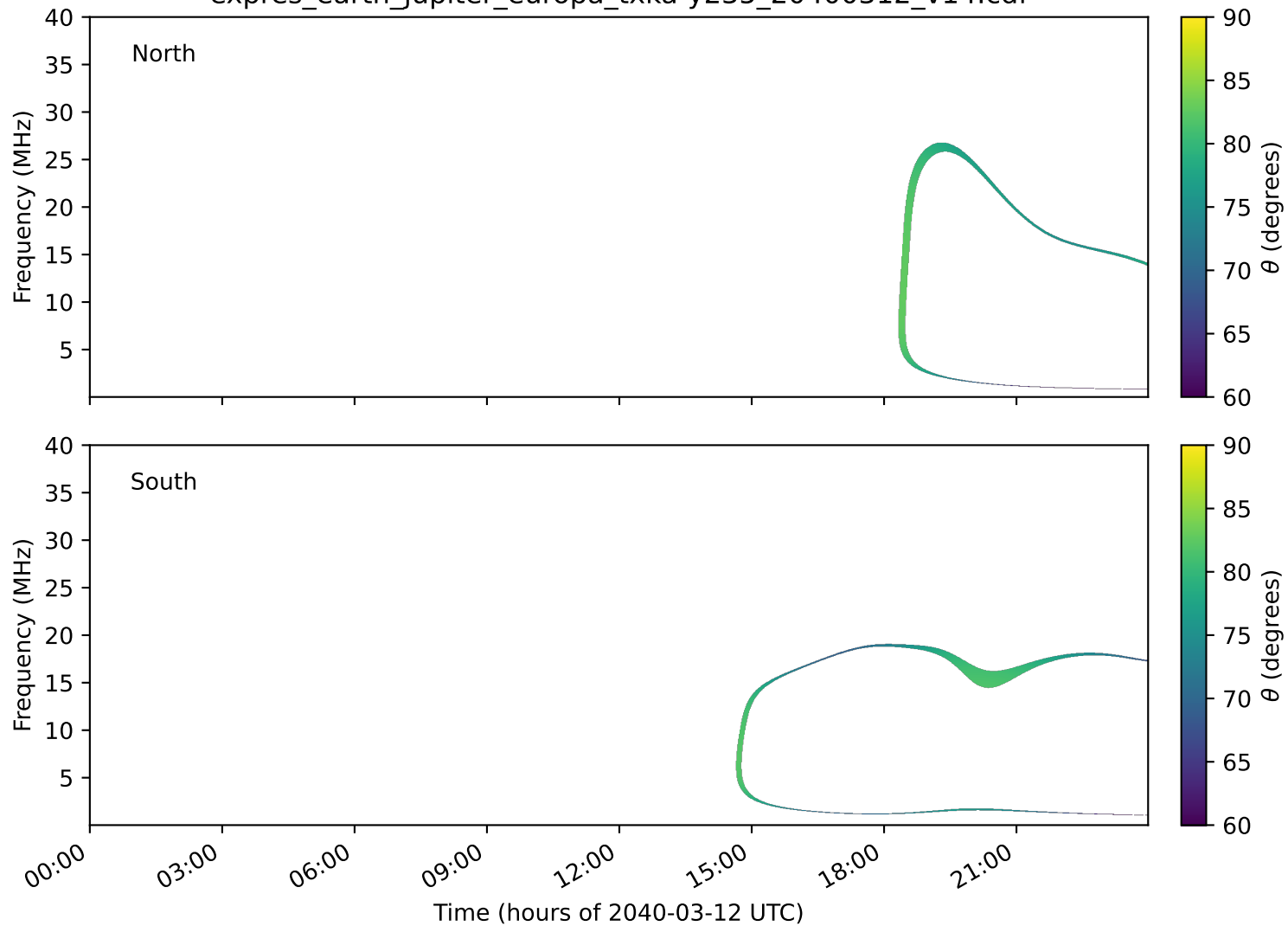
expres_earth_jupiter_europa_txka-y235_20400312_v14.cdf
