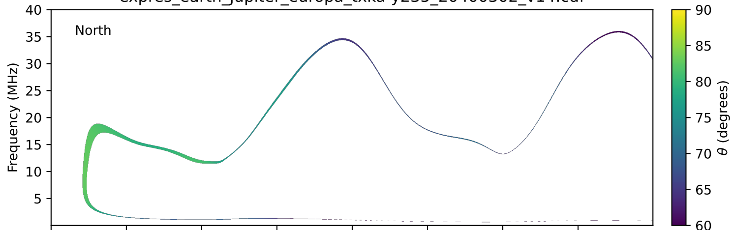
expres_earth_jupiter_europa_txka-y235_20400302_v14.cdf
